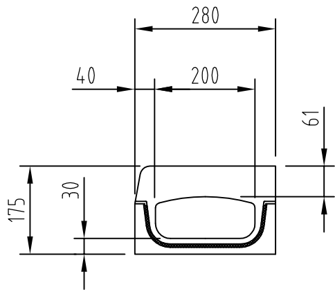
Detail X an Y
